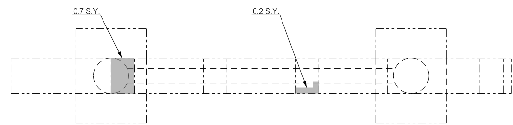
BRIDGE 'A' - WESTBOUND
