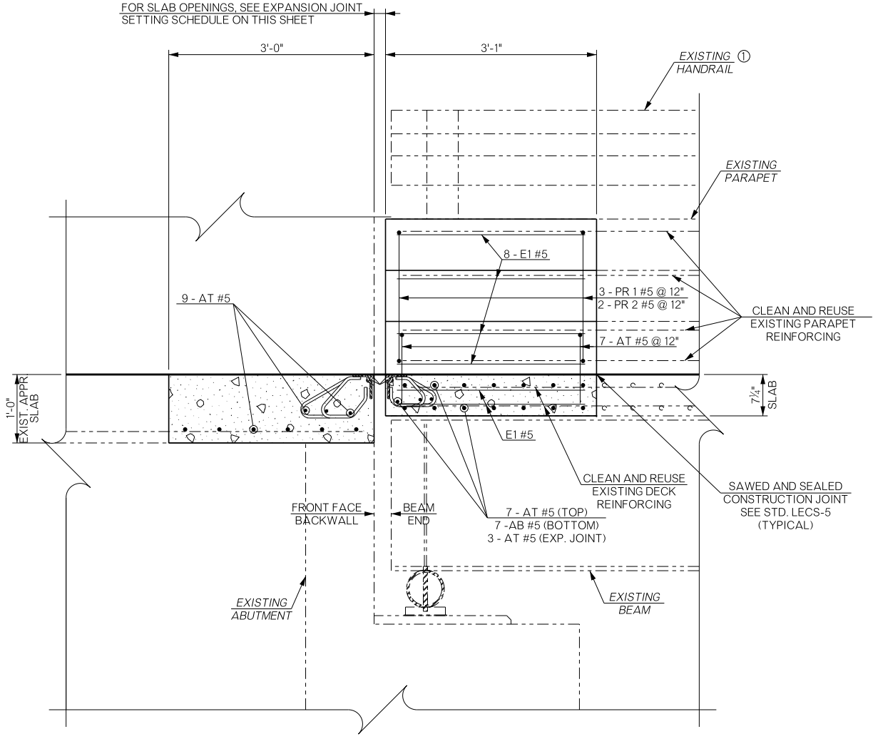
SLAB REPLACEMENT DETAIL AT PARAPET
