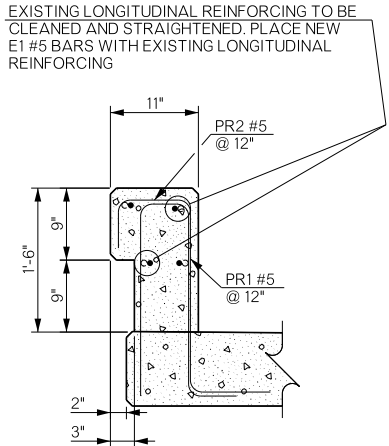
PARAPET DETAIL
