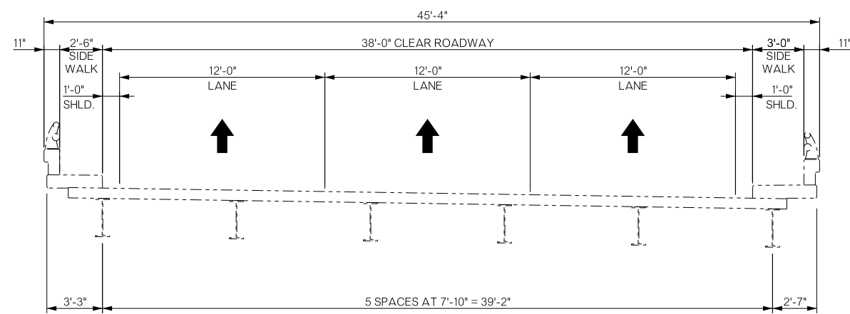
FINISHED BRIDGE
