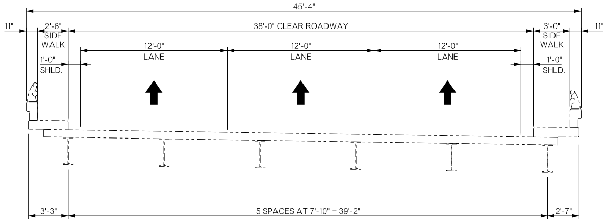
EXISTING BRIDGE
