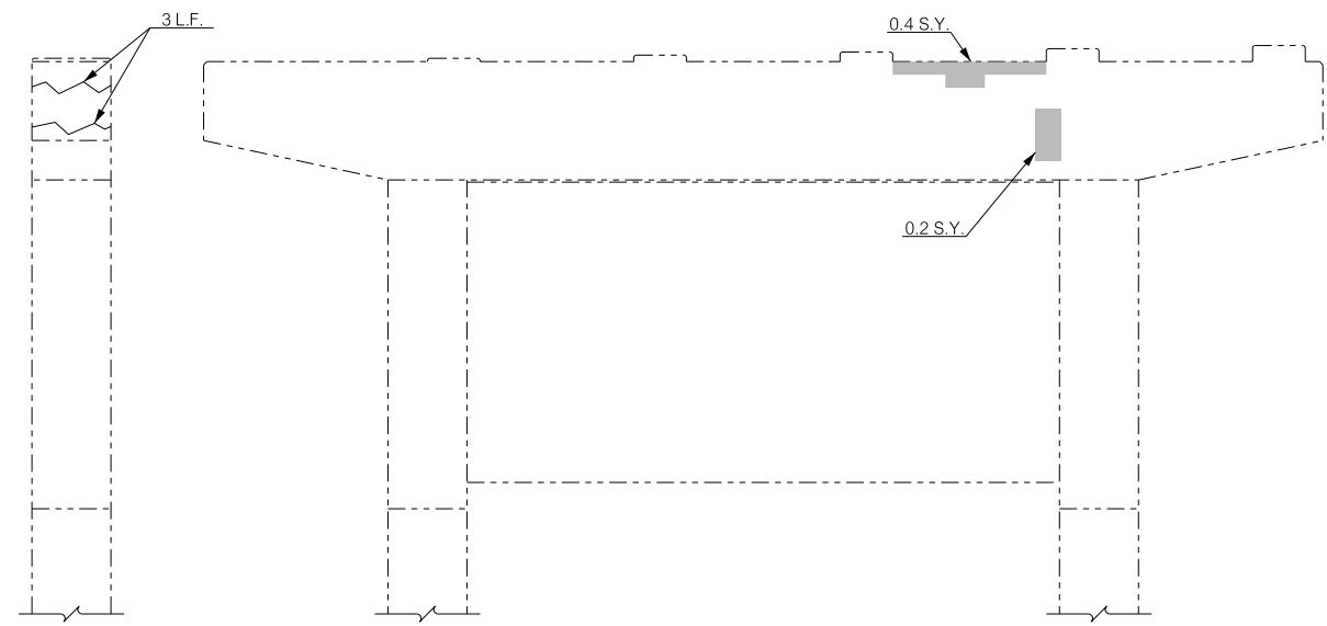
BRIDGE 'B' - PIER NO. 2 SOUTH ELEVATION
