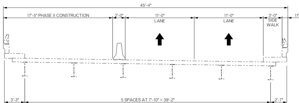
PHASE II
