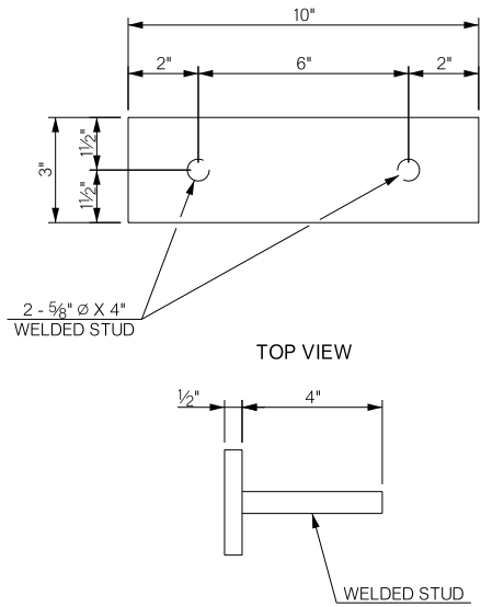
BACKWALL PLATE DETAIL
