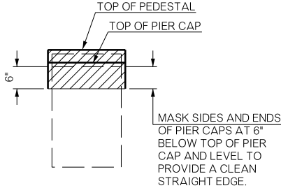
PIERS
