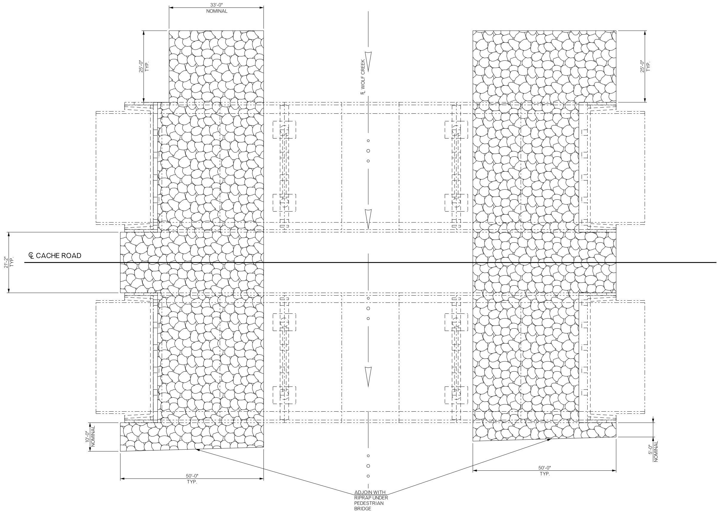
PLAN
