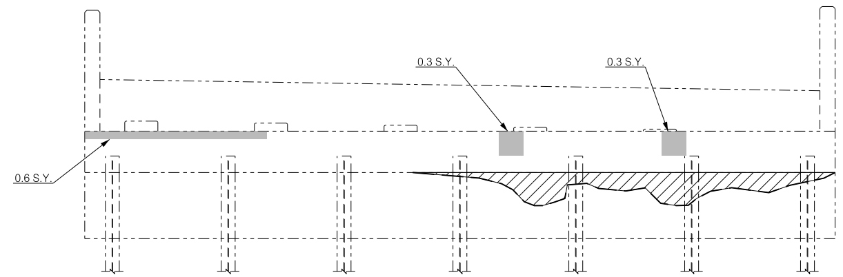
BRIDGE 'A' - WESTBOUND
