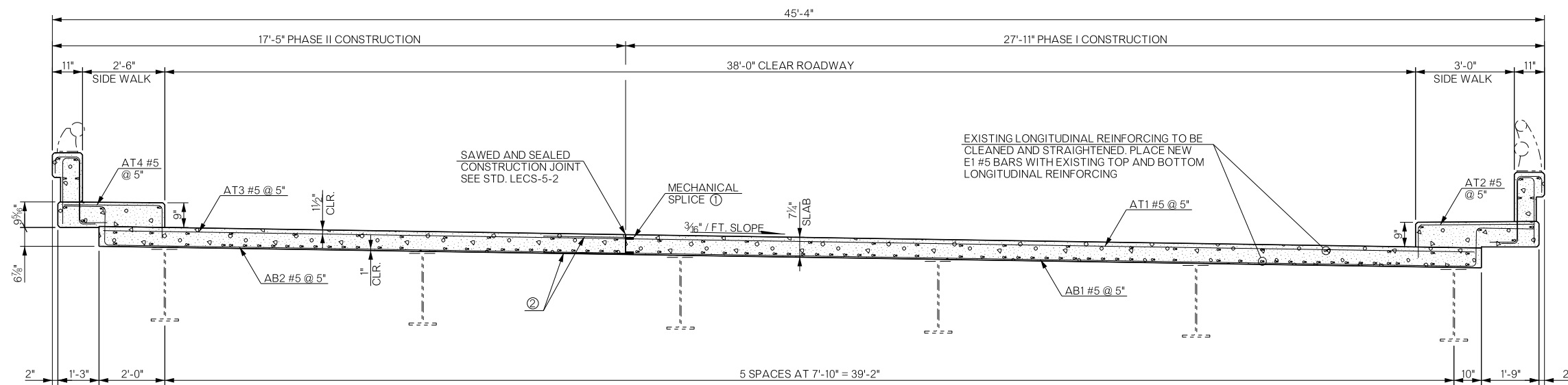
TYPICAL SLAB REPLACEMENT SECTION
