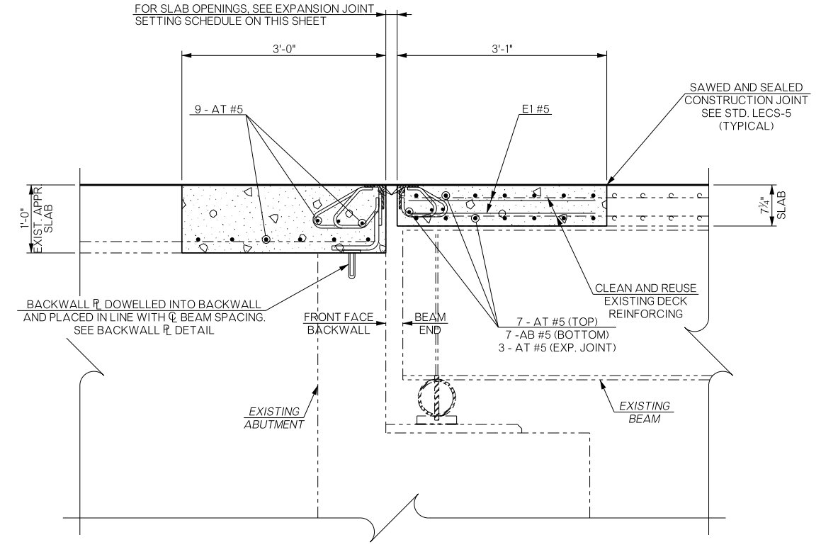
SLAB REPLACEMENT DETAIL AT Q BEAM
