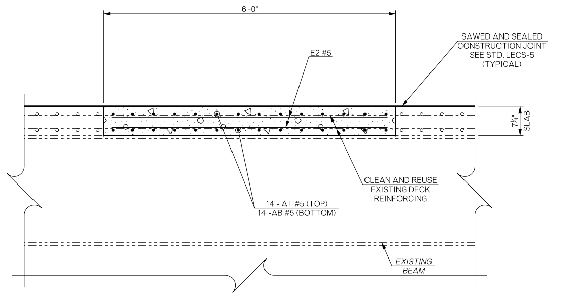
SLAB REPLACEMENT DETAIL
