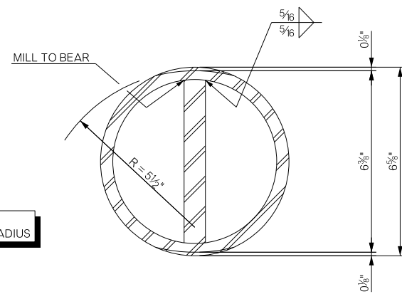
SECTION THRU ROLLER
