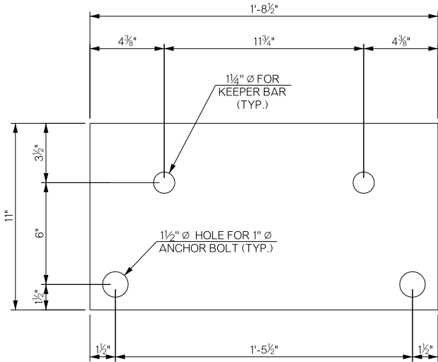
PLAN OF EXPANSION BEARING PLATE
