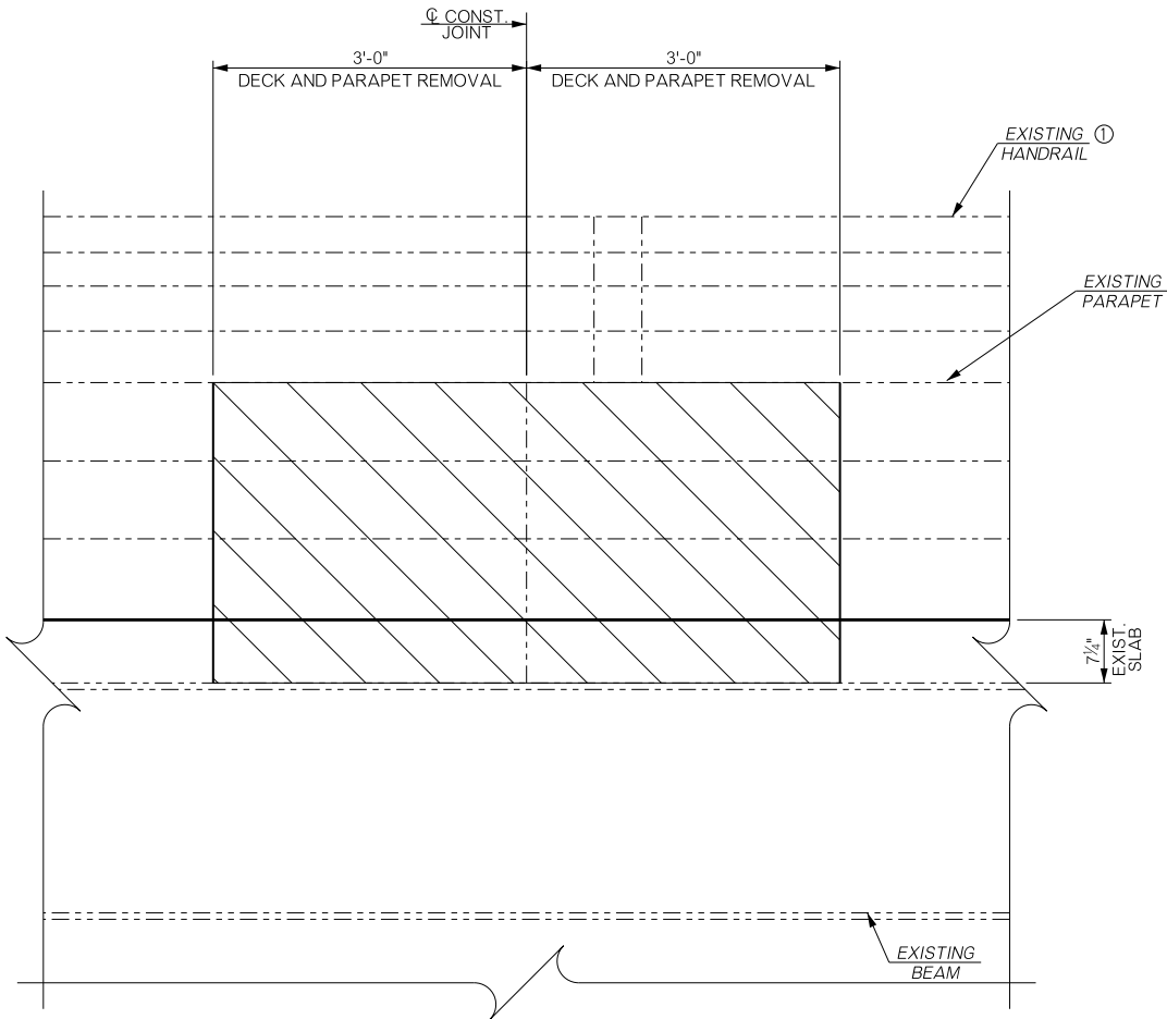
SLAB REMOVAL AT CONSTRUCTION JOINT
