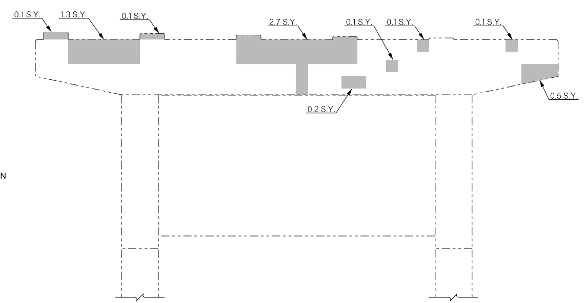
BRIDGE 'A' - WESTBOUND
