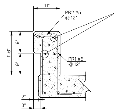
PARAPET DETAIL
