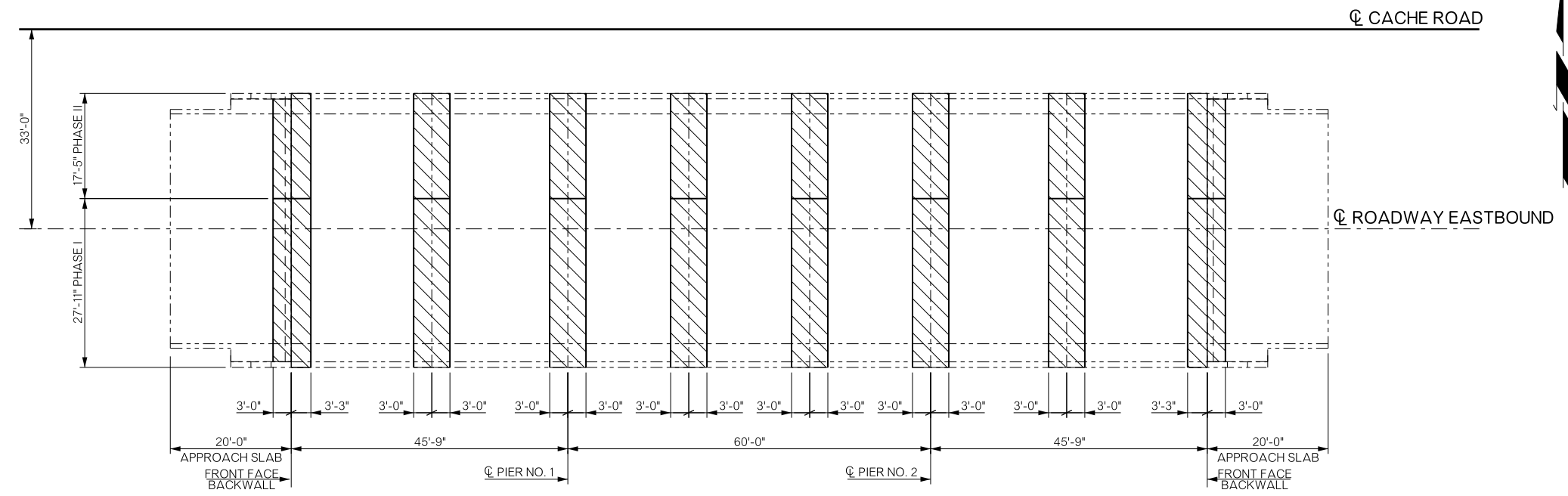
REMOVAL PLAN
