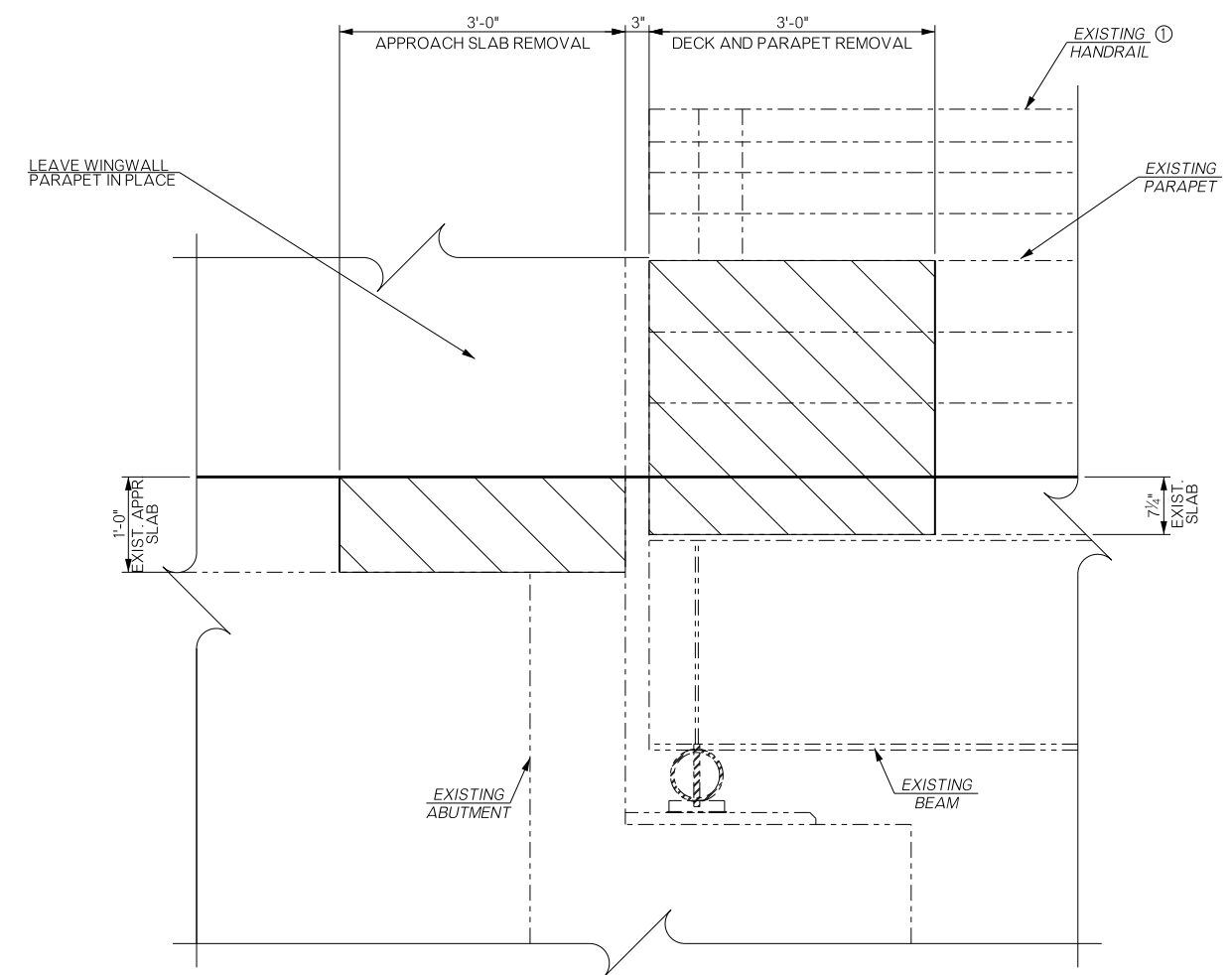
SLAB REMOVAL AT ABUTMENT
