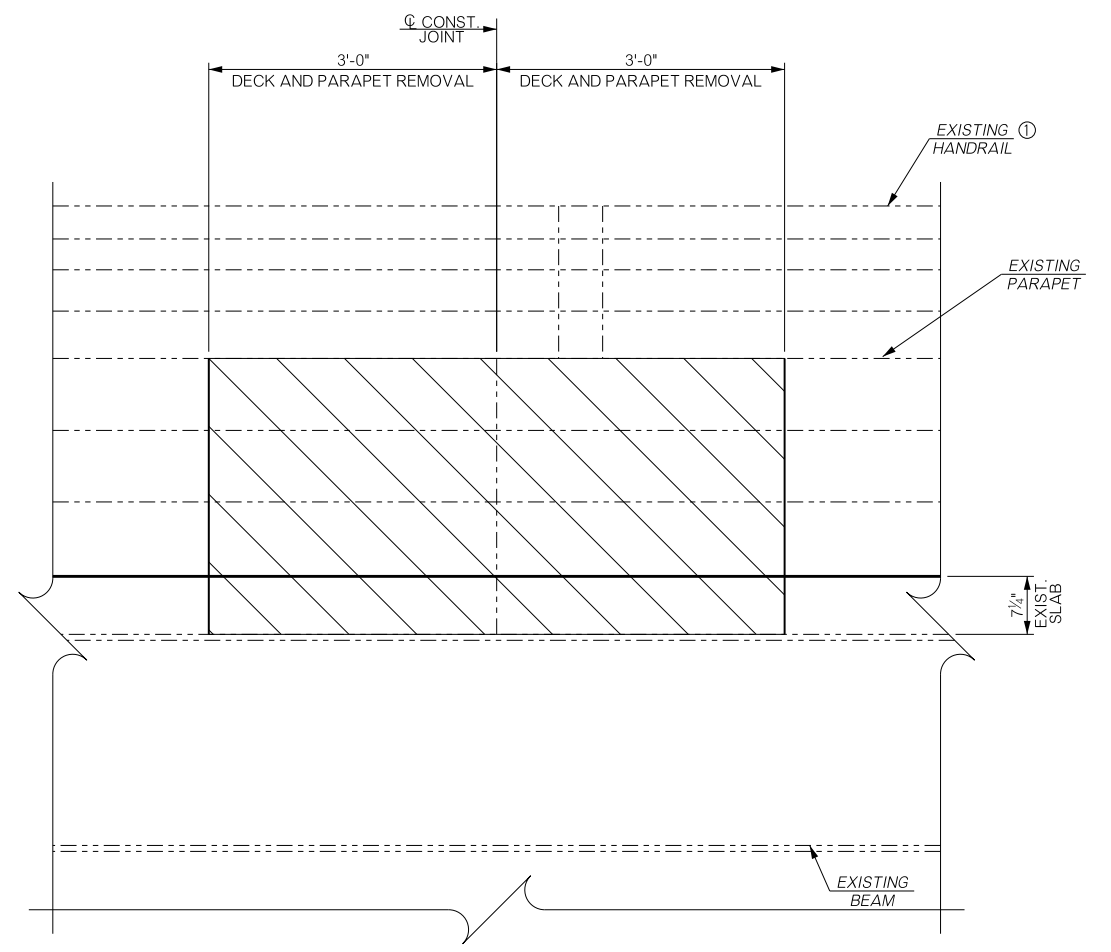
SLAB REMOVAL AT CONSTRUCTION JOINT
