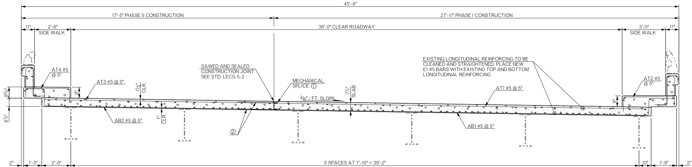
TYPICAL SLAB REPLACEMENT SECTION
