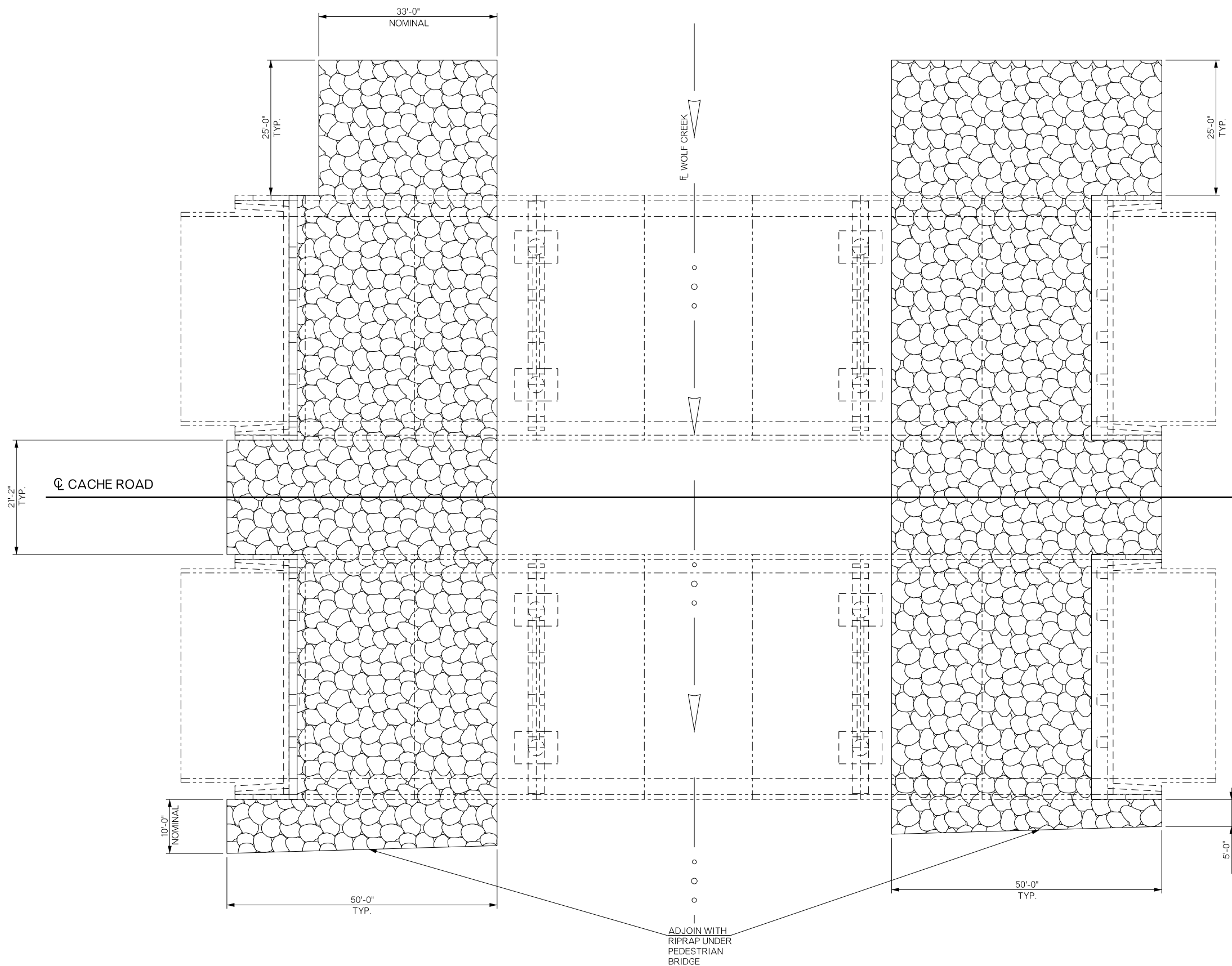
PLAN
