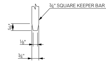
KEEPER DETAIL
