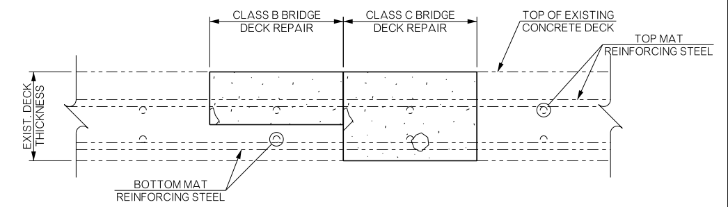
BRIDGE DECK REPAIR DETAIL
