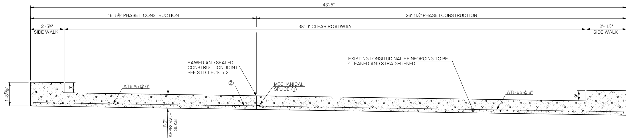
TYPICAL APPROACH SLAB REPLACEMENT SECTION
