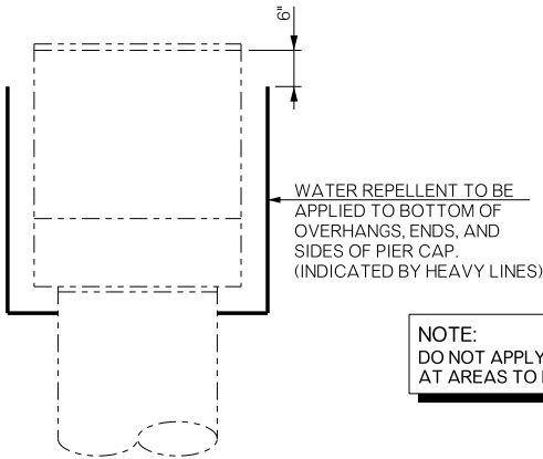
WATER REPELLENT TREATMENT DETAIL
