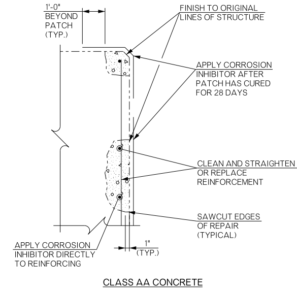
CONCRETE REPAIR DETAILS
