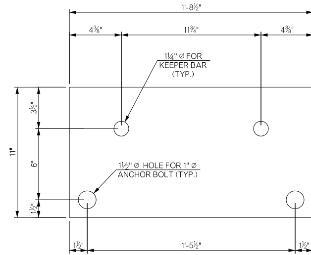
PLAN OF EXPANSION BEARING PLATE
