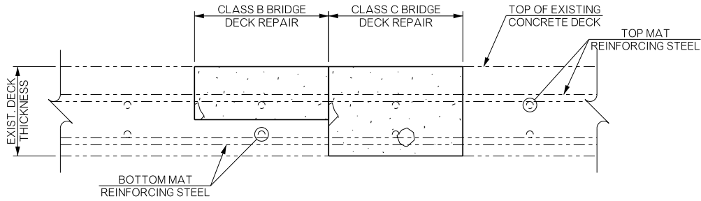
BRIDGE DECK REPAIR DETAIL
