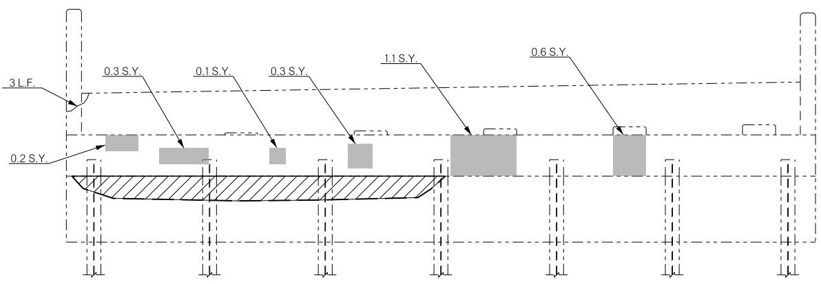
BRIDGE 'A' - WESTBOUND
