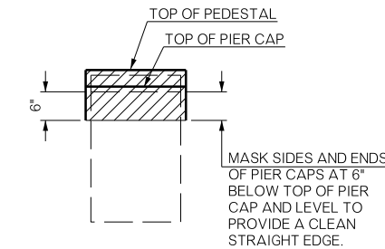
PIERS
