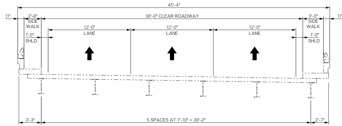
EXISTING BRIDGE
