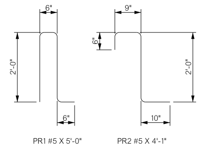
PARAPET DETAIL
