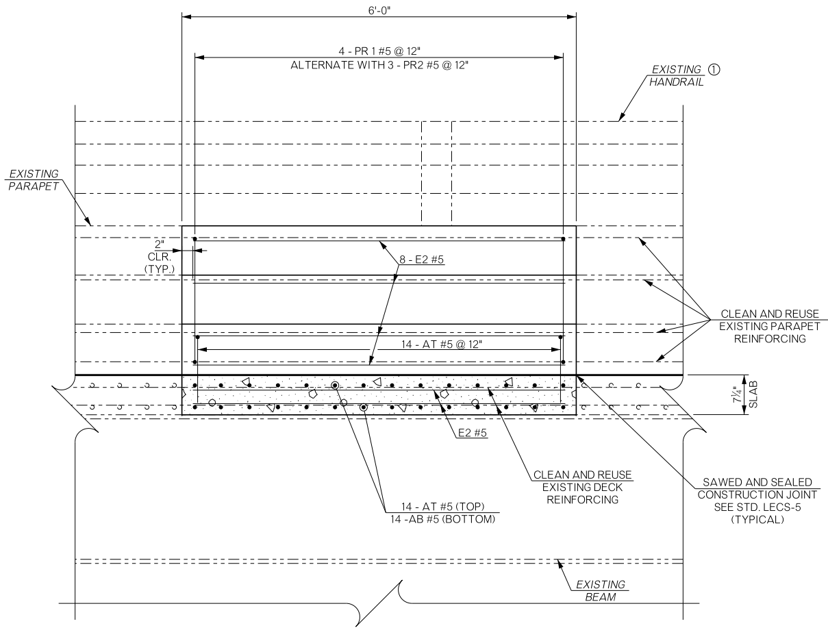
SLAB REPLACEMENT DETAIL AT PARAPET
