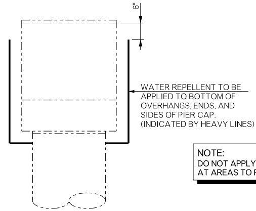
WATER REPELLENT TREATMENT DETAIL
