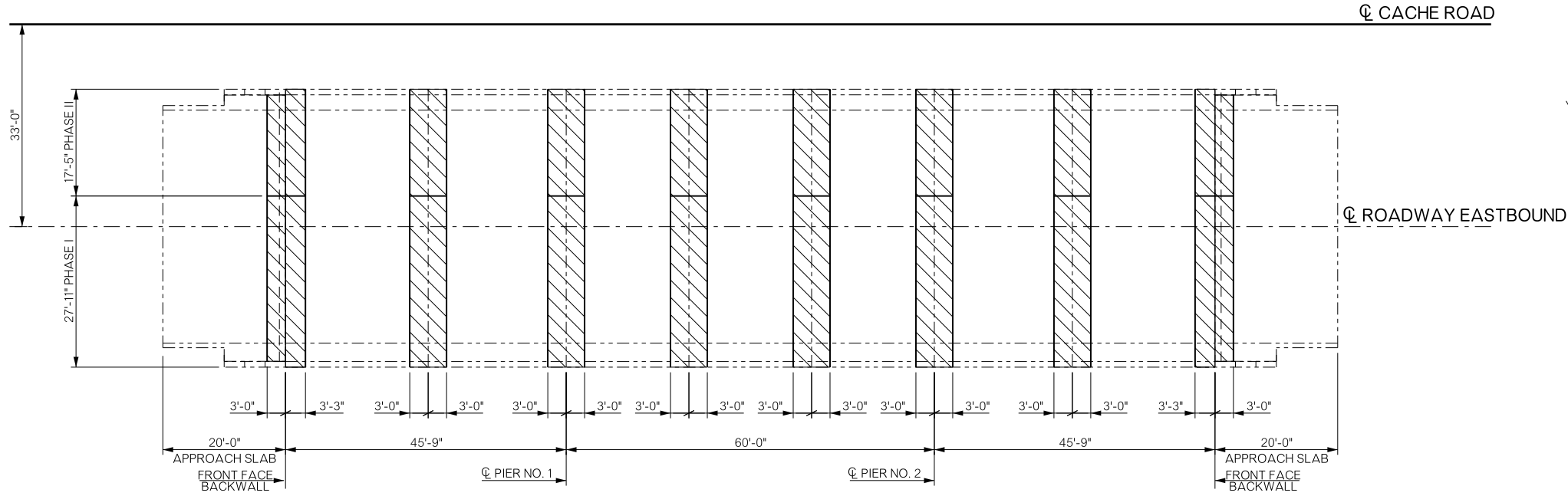
REMOVAL PLAN
