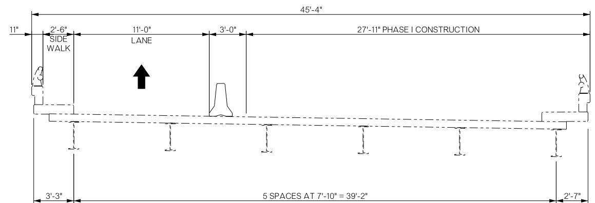
PHASE I
