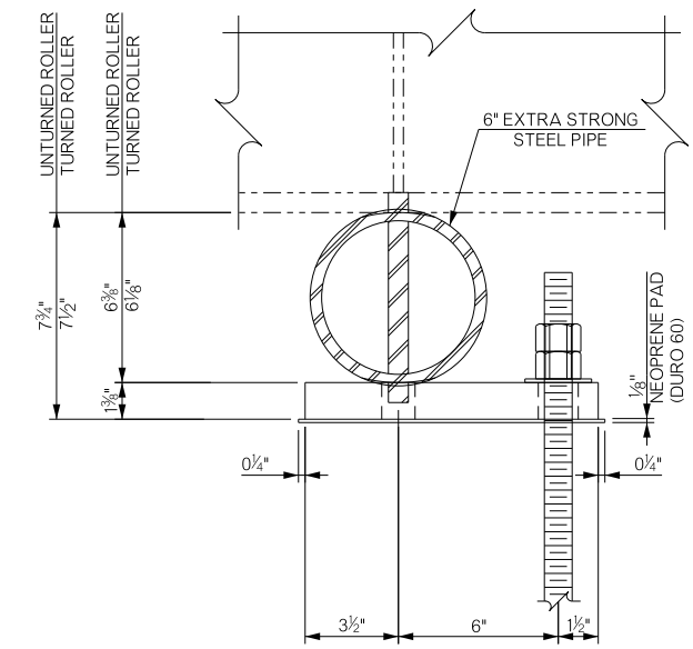
END VIEW
